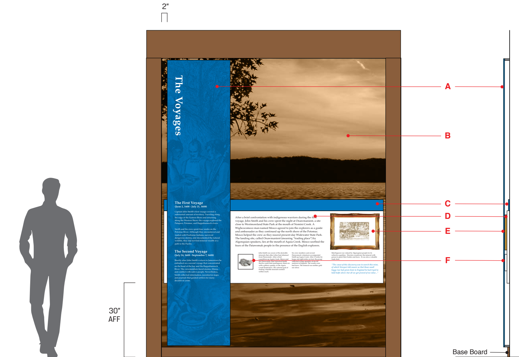
1 EXHIBIT BAY 2 Mounting Elevation SCALE: 1/2"=1'-0"
